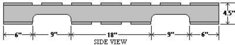
SIDE VIEW
